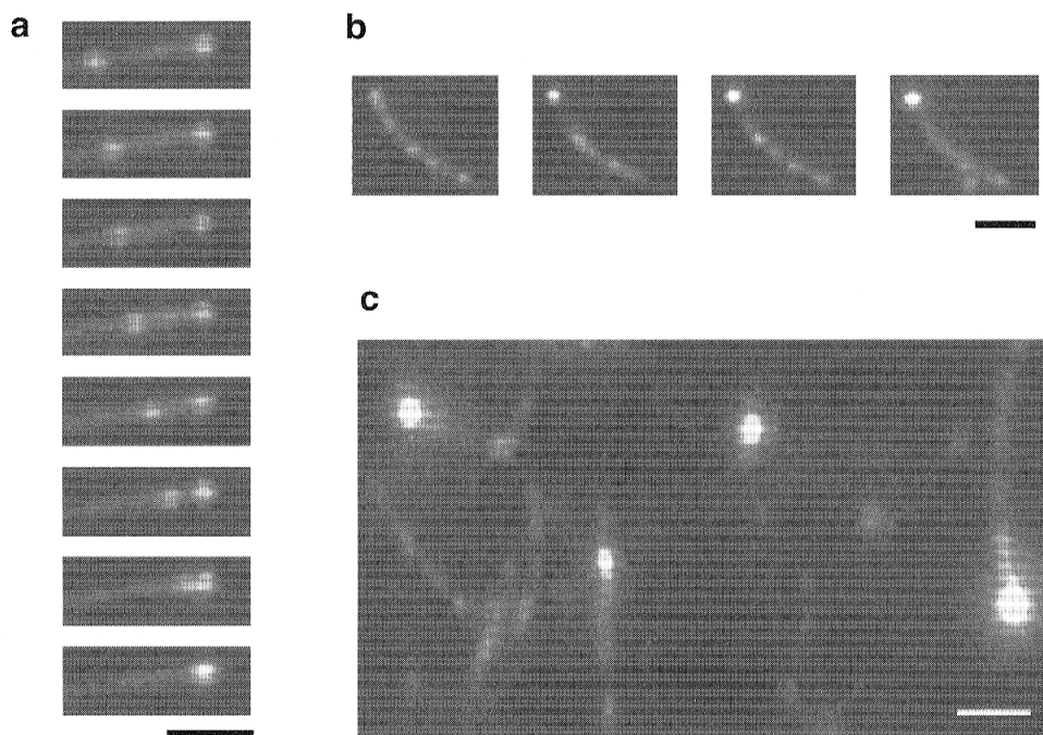
FIG. 2. Processive movement by individual BMV molecules along actin filaments. (a) Successive video images at 0.5-s intervals showing processive movement by a single molecule of BMV along a fluorescent actin filament. The actin filament is labeled with RGP. A light spot in the left-hand side is moving toward the stationary light spot at the actin-filament end. KCl: 75 mM. Scale: 2 \mu\text{m} . (b) Successive video images at 2-s intervals. The barbed end of the actin filament is getting brighter with time because of a constant stream of BMV traffic. A chain of light spots are visible on the actin filament labeled with nonfluorescent phalloidine. KCl: 25 mM. Scale: 2 \mu\text{m} . (c) A video image showing bright spots formed 1 min after incubating BMV in the motility-assay cell. The actin filaments are labeled with nonfluorescent phalloidine. KCl: 25 mM. Scale: 2 \mu\text{m} . The camera gain and the offset levels are different between (a), (b) and (c). In (b) and (c), these parameters for imaging are lower than those in (a). Therefore, we cannot compare the spot intensities in the three cases.
