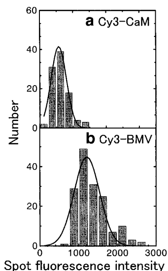
FIG. 1. Distributions of spot intensities (arbitrary units) for (a) Cy3-CaM and (b) Cy3-BMV. The spot intensities were obtained by integrating the intensity over a square (13 \times 13 pixels) enclosing the spot and subtracting a background integrated over the same square after complete photobleaching of Cy3.
