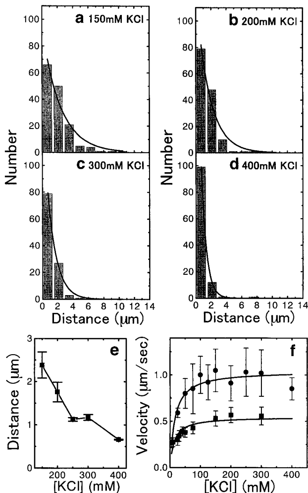
FIG. 3. Processive movement by individual BMV molecules at various ionic strengths. (a–d) Distribution of distances traveled on actin tracks by individual BMV molecules before detachment. Solid curves: exponential fits with length constants, 2.39 \mu\text{m} (a), 1.76 \mu\text{m} (b), 1.17 \mu\text{m} (c), and 0.66 \mu\text{m} (d). The average travel distances are plotted as a function of [KCl] in (e). (f) The rate, as a function of [KCl], of actin-filament translation propelled by large ensembles of BMV (closed squares), and the rate, as a function of [KCl], of processive movement by individual BMV molecules along their actin tracks (closed circles).
