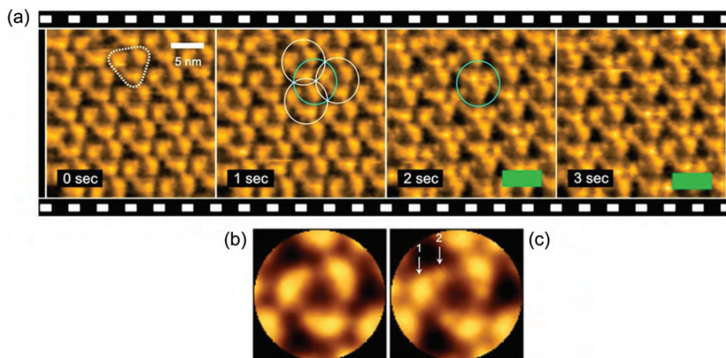
Fig. 4. Structural change in bR induced by light absorption. (a) Successive high-speed AFM images of the cytoplasmic surface of D96N bR in dark and illuminated conditions, captured at 1 fps. The green bars at 2 and 3 s indicate illumination of 532 nm green light with an intensity of 0.5 \mu\text{W} . A bR trimer is highlighted by the white triangle in the image at 0 s. In the image at 1 s, three adjacent trimers are encircled with white circles, while a trefoil comprised of three nearest-neighbor monomers, each belonging to one of the encircled trimers, is indicated with the light-blue circle. The same trefoil is encircled in light blue in the images at 2 and 3 s. (b) Averaged AFM image of trimer in dark conditions. (c) Averaged AFM image of trimer under illumination. Under illumination, the protrusion is split into larger (arrow 1) and smaller (arrow 2) sections.
