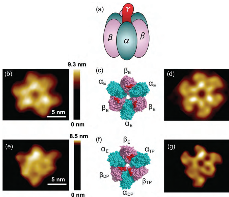
Fig. 2. AFM images of \alpha_3\beta_3 subcomplex at C-terminal surface. (a) Schematic for F_1 -ATPase. (b) Averaged AFM image obtained in nucleotide-free condition. (c) C-terminal surface of crystal structure of nucleotide-free \alpha_3\beta_3 subcomplex. (d) Simulated AFM image of (c). (e) Averaged AFM image obtained in 1 mM AMP-PNP. (f) C-terminal surface of crystal structure of \alpha_3\beta_3 subcomplex obtained in ATP. (g) Simulated AFM image of (f).
