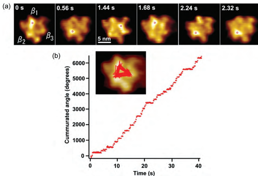
Fig. 3. Rotary propagation of conformational change of \alpha_3\beta_3 subcomplex at C-terminal surface. (a) Successive images of C-terminal surface of \alpha_3\beta_3 subcomplex in 2\ \mu\text{M} ATP, captured by HS-AFM at 12.5 fps. The highest pixel position in each image is marked with the red circle. (b) Time evolution of the cumulated angle of the highest pixel. The inset shows a trajectory, superimposed on an AFM image, of the highest pixels corresponding to the high protrusions of \beta subunits in the open state.
