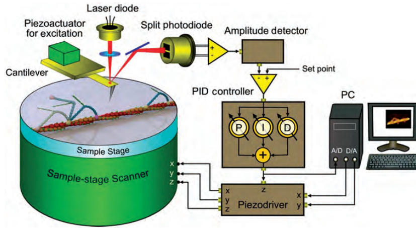
Fig. 1. Schematic of tapping-mode AFM setup. The cantilever is vertically oscillated at its first resonant frequency. The cantilever deflection is detected by the optical beam deflection detector comprised of the laser diode and the split photodetector. The differential signal from the split photodetector is converted into an amplitude signal by the amplitude detector. The detected amplitude signal is compared with the predetermined set point, and their difference (error signal) is processed (mainly integrated) by the PID feedback controller to produce a driving signal for displacing the z-scanner so that the error signal approaches zero. By this control, the oscillation amplitude of the cantilever (and hence, the vertical tip-sample interaction force) is mostly maintained constant during the lateral scanning of the sample stage. The D/A converters implemented in the PC output drive signals to laterally move the sample stage, while the A/D converter records the feedback controller output representing the sample height.
