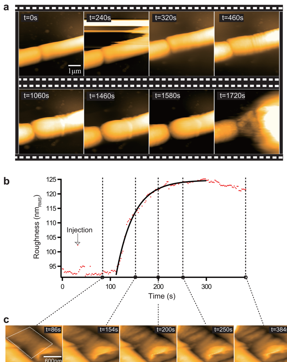
Figure 44. Process of lysozyme-induced bacteriolysis captured by HS-AFM. (a) Time-lapse images of bacteriolytic process of B. subtilis subjected to lysozyme. Lysozyme was injected at t = 240\text{ s} . Scan range, 5 \times 5\text{ }\mu\text{m}^2 ; imaging rate, 0.05\text{ fps} ( 20\text{ s/frame} ); pixels, 256 \times 256 . (b) Time course of RMS roughness of the outer surface of B. subtilis subjected to lysozyme. Lysozyme was injected at t = 32\text{ s} . Solid line shows the result of best fitting (time constant, \tau = 36.8\text{ s} ) by a single exponential function for the time course between t = 112\text{ s} and t = 300\text{ s} . (c) Corresponding clips of successive AFM images of the outer surface of B. subtilis at different time lapses. Values of RMS roughness were calculated for the area encircled by the white broken line shown in the image at t = 86\text{ s} .
