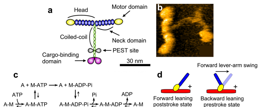
Figure 6. Structure of myosin V, actomyosin ATPase reaction scheme, and prevailing view on conformational states of myosin. (a) Schematic of molecular structure of myosin V. (b) AFM image of myosin V. (c) Reaction scheme of actomyosin ATPase. (d) Schematic for backward leaning prestroke and forward leaning poststroke conformations. The mark “+” indicates the plus end of an actin filament (red). The motor domain (yellow) binds to an actin filament in the same orientation, in both conformational states, while the neck (blue) is leaned in different directions. The forward lever-arm swing is supposed to occur on the actin-bound head when Pi is released from myosin. The backward lever-arm swing is supposed to occur on the detached head when ATP is hydrolyzed to ADP+Pi.
