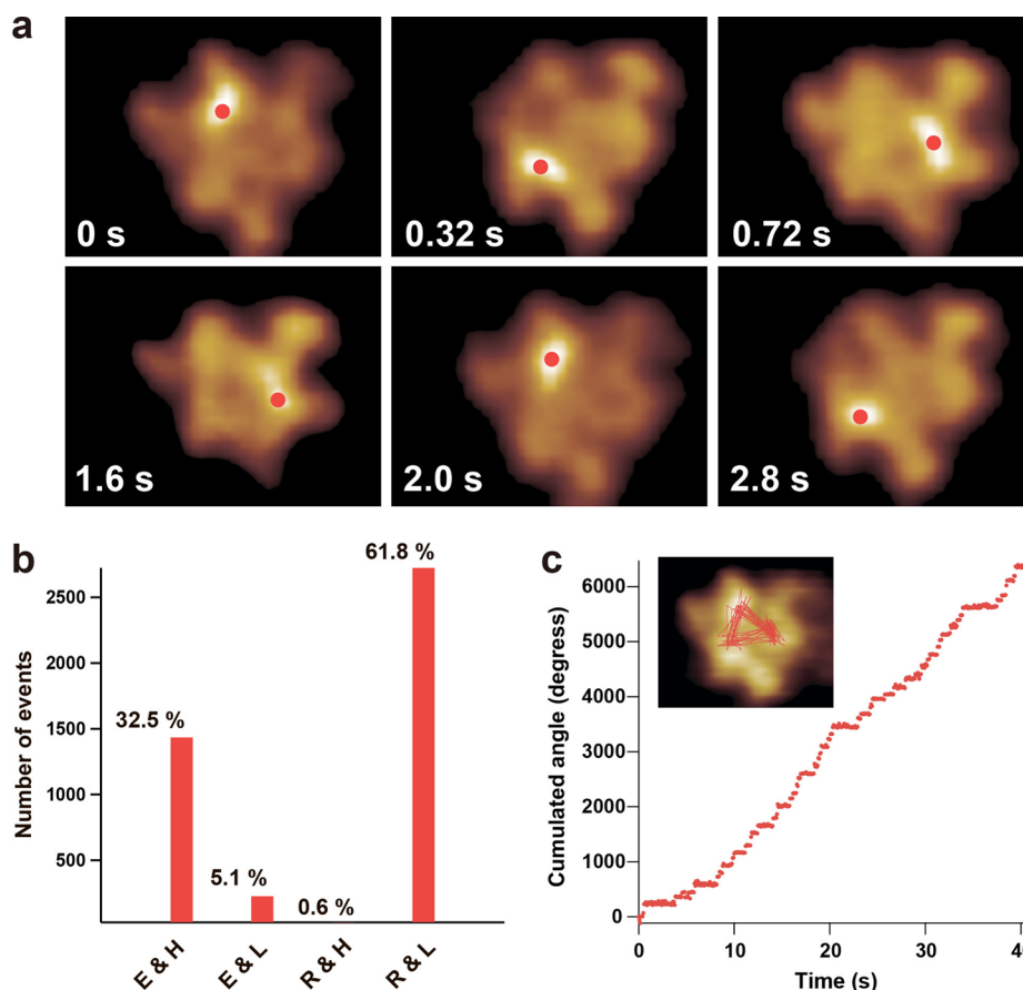
Figure 14. HS-AFM imaging of \alpha_3\beta_3 subcomplex in ATP. (a) Clips of successively captured HS-AFM images of the C-terminal side of \alpha_3\beta_3 subcomplex in 2 \mu\text{M} ATP (imaging rate, 12.5 fps). The highest pixel in each image is indicated by the red circle. (b) Tight correlation between two types of conformational changes in \beta subunits observed in ATP; different heights of protrusion (“H”, high; “L”, low) and extended/retracted (“E”/“R”) conformations of the distal region. (c) Time course of cumulated angle of the highest pixel. The inset shows a trajectory, superimposed on an AFM image, of the highest pixels corresponding to the high protrusions of extended \beta subunits (412 frames). The center of rotation is defined by the averaged X- and Y-positions of the highest pixels, and the cumulated angles are calculated relative to the first frame.
