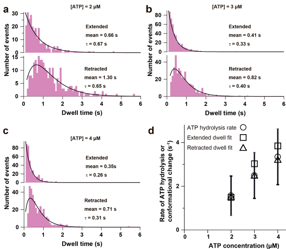
Figure 16. Kinetics analysis of conformational change of \alpha_3\beta_3 subcomplex. Histograms of dwell times for the E (top) and R (bottom) states in various concentrations of ATP (a, 2 \mu M, n = 266; b, 3 \mu M, n = 426; c, 4 \mu M, n = 374). Dwell time distributions for the E state fit well with single exponential decay functions (solid lines on top). The distributions for the R state fit with functions representing consecutive reactions with two identical time constants: A \times t \times \exp(-t/\tau) (solid lines on bottom). (d) ATP concentration dependence of the rate of conformational change of \beta subunit determined by fitting the dwell-time histograms of the E and R states, shown in (a)–(c), and the initial rate of ATP hydrolysis determined by biochemical assay at three different ATP concentrations.
