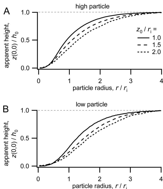
FIG. 5. Calculated apparent height of a single cylindrical particle on a planar surface in a SICM image, as a function of particle radius r . Actual particle heights (a) h_0 = r_i and (b) h_0 = r_i/2 . For r \geq 3r_i the apparent height closely matches the actual height. For r < 3r_i the apparent height is significantly decreased and becomes zero for r=0 . The different traces represent different pipette-sample distances z_0 .
