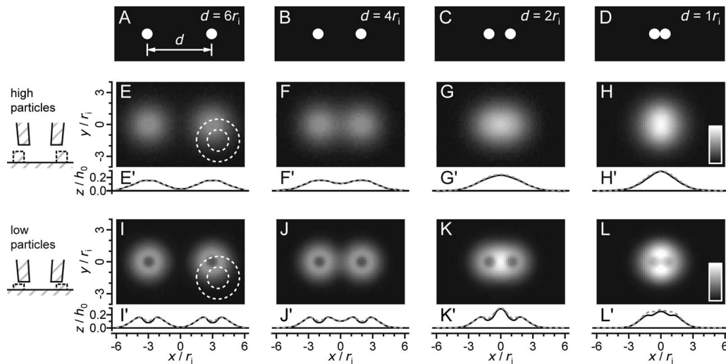
FIG. 6. Calculated topography images of two cylindrical particles of radius r = r_i/2 on a planar surface. [(a)–(d)] Actual topography. [(e)–(h)] Calculated topography images for two high particles, h_0 = r_i , and a large pipette-sample distance, z_0 = 1.6r_i . [(i)–(l)] Images for low particles, h_0 = r_i/2 , and a small pipette-sample distance, z_0 = 0.6r_i . (e) At a large particle distance, d = 6r_i , each high particle is imaged as a single bell shape [black trace in cross section (e')]. This is equivalent to the superposition of two single particle images from Fig. 4(a) [gray dashed trace in (e')]. [(f) and (f')] For a decreasing distance, d = 4r_i , the bell shapes start to overlap and are not resolvable from each other any more for [(g) and (g')] d = 2r_i and [(h) and (h')] d = r_i . (i) At a large particle distance, d = 6r_i , each low particle images as a ring [black trace in cross section (i')]. This is equivalent to the superposition of two single particle images from Fig. 4(e) [gray dashed trace in (i')]. [(j) and (j')] The rings start to overlap for d = 4r_i . [(k) and (k')] For a smaller particle distance the rings overlap in the center between the particles. [(l) and (l')] For an even smaller distance the largest overlap is above and below the x-axis. In this case, the image appears as if two particles rotated by 90^\circ were present. The color bars indicate a height range of 0.0 – 0.3h_0 . The pipette tip opening is outlined dashed in (e) and (i).
