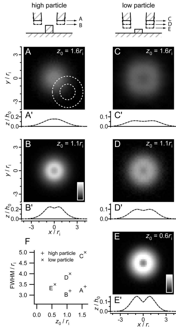
FIG. 4. Calculated topography images of a single cylindrical particle of radius r = r_i/2 on a planar surface. (a) A high particle, h_0 = r_i , imaged at a large pipette-sample distance, z_0 = 1.6r_i , appears blurred in the image. The corresponding cross section (a') is bell-shaped with a height of 0.16h_0 and a FWHM of 3.2r_i . [(b) and (b')] Decreasing the pipette-sample distance, z_0 = 1.1r_i , causes an increase in the apparent height and a dip to appear in the center. [(c) and (c')] A low particle, h_0 = r_i/2 , results in an overproportionally smaller apparent height and is always imaged as a ring, both at a large pipette-sample distance, z_0 = 1.6r_i , and at smaller pipette-sample distances, [(d) and (d')] z_0 = 1.1r_i and [(e) and (e')] z_0 = 0.6r_i . The color bars indicate height ranges of 0.0 – 0.32h_0 [(a) and (b)] and 0.0 – 0.16h_0 [(c)–(e)], respectively. The pipette tip opening with inner radius r_i and outer radius r_o = 2r_i is outlined as dashed circles in (a). (f) FWHM values as a function of pipette-sample distance, z_0 , for the high and low particles, respectively. The FWHM decreases with the pipette-sample distance to a minimum value of about 3.0r_i .
