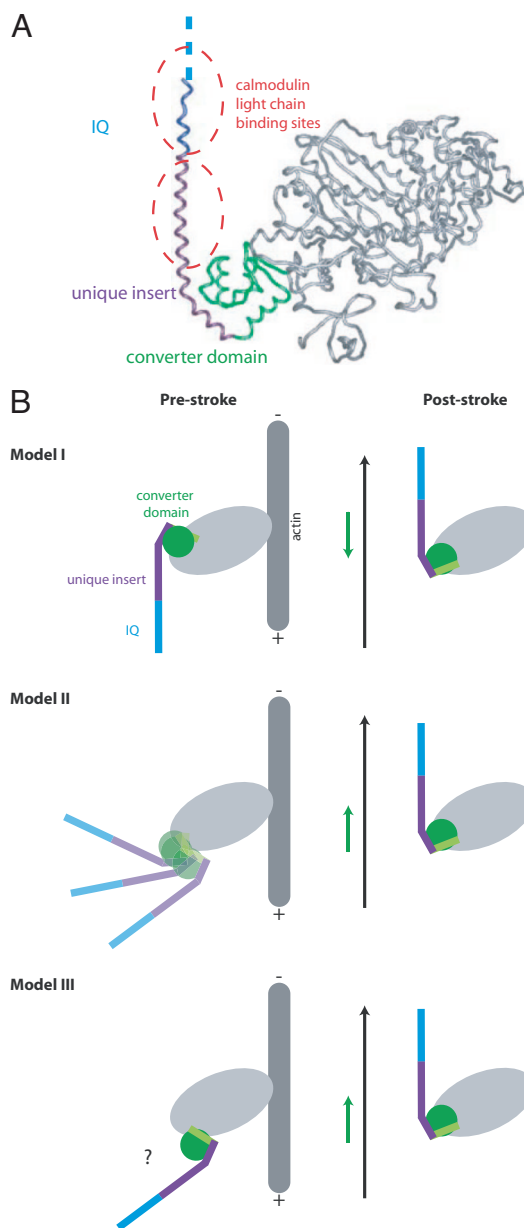
Fig. 1. The pre- and poststroke conformations of myosin VI. (A) Poststroke x-ray crystal structure (12). A class-specific insertion (purple) emerges from the final helix of the converter domain (green) and serves to redirect the lever arm toward the (–) end of the actin filament. The IQ domain (blue) is not completely resolved in the structure and is followed by a flexible domain of unknown structure that may extend the lever arm (see Discussion ). Two calmodulin light chains (not shown) bind to the extended helix formed by the IQ domain and the distal portion of the unique insert at the locations indicated by the dashed ovals. (B) Speculative models for the myosin VI power stroke [models I and II adapted from Ménétrey et al. (12)]. Light chains are omitted for clarity. The final helix of the converter domain is indicated in light green. Black arrows indicate the net motion of the tip of the lever arm, and green arrows indicate the net motion of the converter domain. In model I, the converter domain moves toward the (+) end of the actin filament while the redirected lever arm moves toward the (–) end. To explain the large stroke size, the converter domain must be rotated in the prestroke state relative to its position in known prestroke structures of (+)-end-directed myosins. In model II, the power stroke consists of a disorder-to-order transition in which the average position of the converter domain moves toward the (–) end. Another class of models (model III) involves a rigid motion of the converter domain toward the (–) end. Other possibilities (not shown) might include a disruption of the interface between the unique insert and the converter domain.
