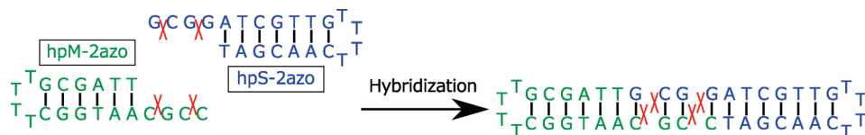
FIGURE 5. Hybridization between two hairpins, hpM-2azo and hpS-2azo. The X denotes azobenzenes.
