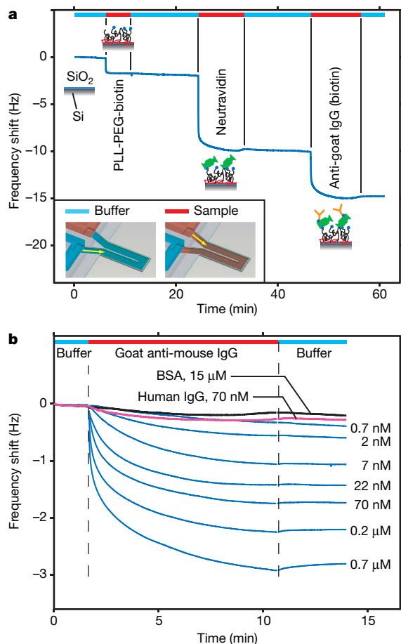
Figure 3 | Resonance frequency shifts caused by accumulation of proteins inside the cantilever. a , Antibodies to goat IgG are immobilized on the native silicon dioxide surface of the suspended microchannel resonator in three steps, as illustrated by the pictograms along the frequency trace: electrostatic adsorption of poly(ethyleneglycol)-biotin grafted poly-L-lysine (PLL-PEG-biotin, 1 mg ml -1 ), binding of Neutravidin (0.5 mg ml -1 ), and attachment of biotinylated antibodies (0.5 mg ml -1 ) to the Neutravidin. The mass increase at each step can be followed in real time (1 Hz ≈ 300 fmol cm -2 for 150 kDa IgG molecules). One bypass channel was continuously rinsed with phosphate buffered saline (PBS) while the other bypass contained the sample. During the injection interval (red), the bypass holding the sample was pressurized, and during rinse cycles (blue), the pressure difference was reversed, as shown in the inset at the bottom of the panel. b , Goat anti-mouse IgG was injected at concentrations from 0.7 nM to 0.7 μM (blue traces). Between measurements, the surface was regenerated by injecting 200 mM glycine (HCl; pH 2.5), which dissociated the analyte while preserving the activity of the antibodies. Control injections with no IgG (black) or human IgG (red) showed very low levels of non-specific binding.
